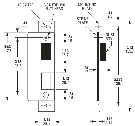
4901-01 FLAT with Dust Box & Mounting Plate
