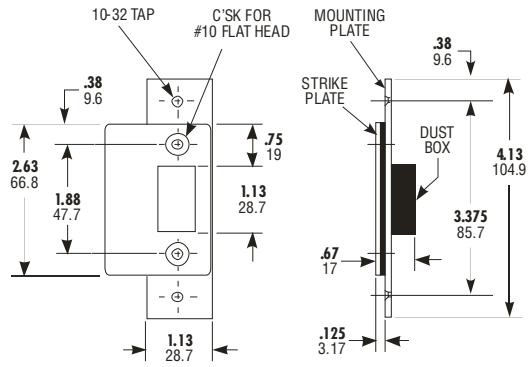
4902-01 FLAT with Dust Box & Mounting Plate
