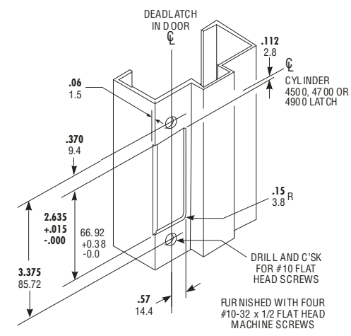
4902-01 FLAT with Dust Box & Mounting Plate
