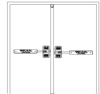
Double Doors with Key Removable Mullion
