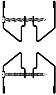
LT-B1 3/8" Glazing Pocket for 3/4" Glass
