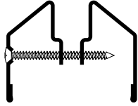
LT-B1 3/8" Glazing Pocket for 1/4" Glass
