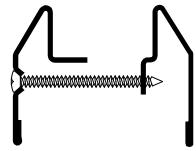
LT-B4 1 1/16" Glazing Pocket for 7/8" to 1" Glass
