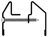
LT-B3 13/16" Glazing Pocket for 5/8" to 3/4" Glass
