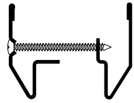
LT-B2 9/16" Glazing Pocket for 3/8" to 1/2" Glass
