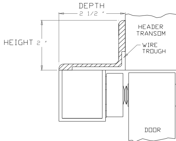
1194 ANGLE BRACKET
