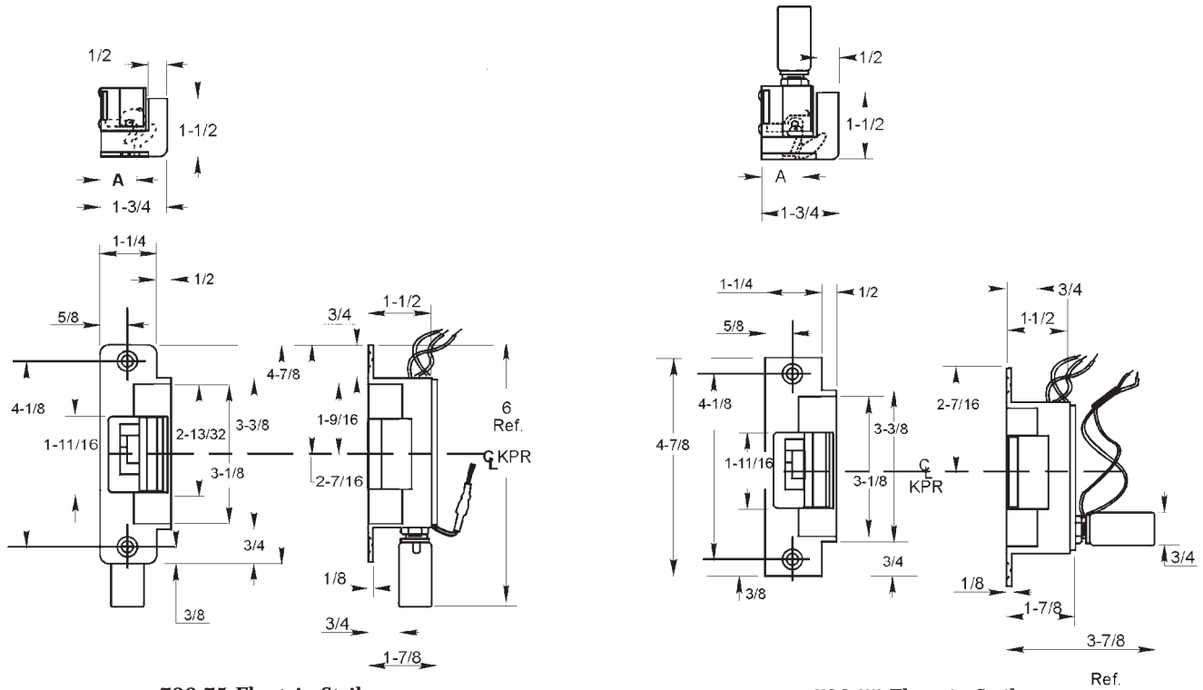
722-75 Electric Strike
