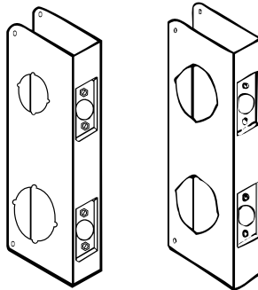
CW-486 Hole Sizes 1-1/2" over 2-1/8"
