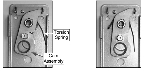
Fig. 7. Torsion Spring connected—"Always Armed" mode (left) and disconnected—"On/Off" mode (right). See CONFIGURATION on page 2
