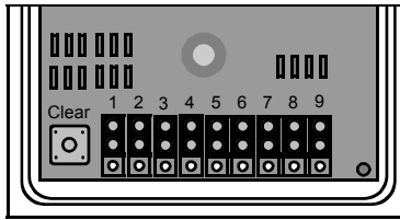
Fig. 6. Jumper Positions. Jumpers 1-9 shown in factory default positions—all jumpers "up".
