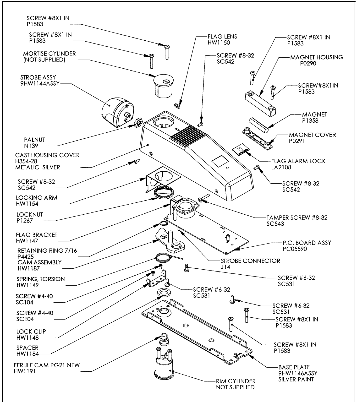
Fig. 7 Exploded view with part numbers
